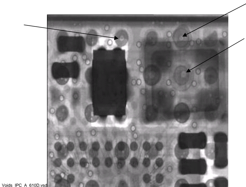
Figure Two: X-ray Picture Showing Voids Conforming to IPC-A-610D
